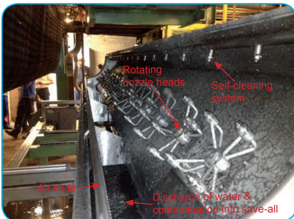
Cleaning Head in Maintenance Position
